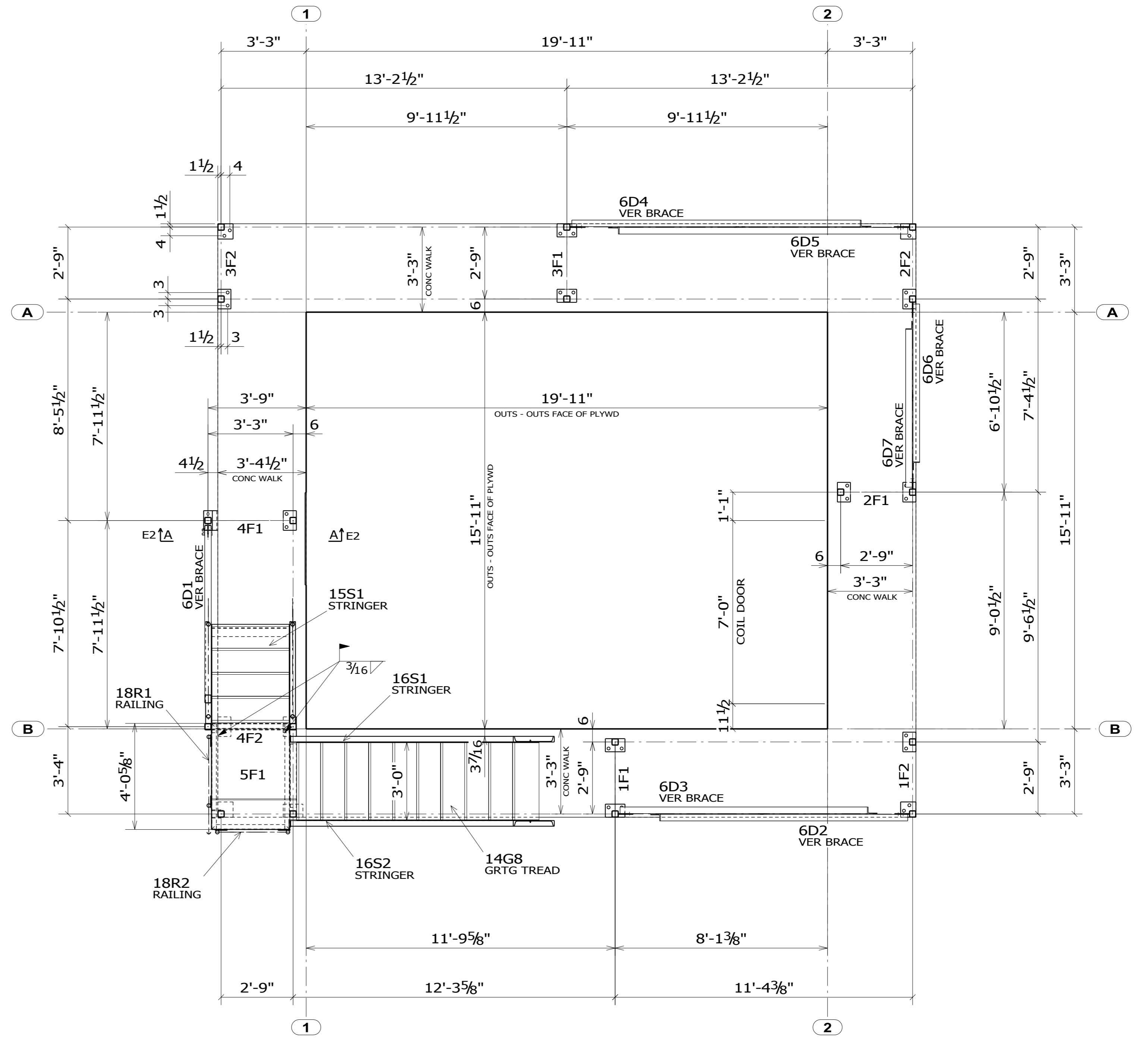
EL. 0'-0"
